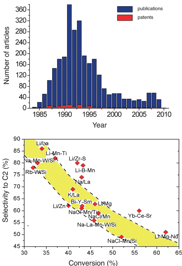
Figure 3. Scientific activities in the oxidative coupling of methane (OCM) as a function of time. In the lower graphic the most successful catalysts are displayed in a conversion–selectivity diagram.
