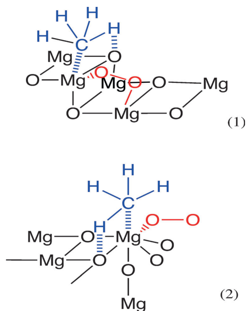
Figure 8. Intermediate steps for the activation of methane on MgO: (1) on a free (100) step, (2) on a (111) O-terminated step. The hydroxylation is not shown.
