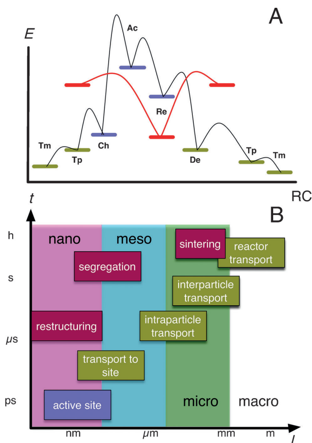
Figure 1. Dimensions in catalysis: A) Change in energy (E) of a catalytic system with respect to the reaction coordinate (RC) for the basic individual steps: Tm: transport macroscopic, Tp: transport in pores or solvation shells, Ch: chemisorption, AC: activation (dissociation), Re: reaction, De: desorption, dissociation. The energy changes in red denote the impact of the reaction on active centers that are taken here to be adaptive. B) Space–time scales for a heterogeneous catalytic process: blue: the molecular reaction, red: chemical dynamics on the catalyst, green: transport processes of the reactants. The vertical bars indicate often-used terms for the spatial dimensions.
