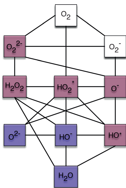
Figure 2. A simple reaction network for the activation of oxygen. Hydrogen and an unnamed electron donor are needed. Red denotes the formal oxidation state -1 and blue the oxidation state -2 .
