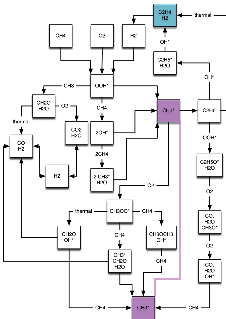
Figure 5. Simplified reaction network for the activation of methane over MgO. The double appearance of “CH 3 ” is for clarity and has no mechanistic purpose.
