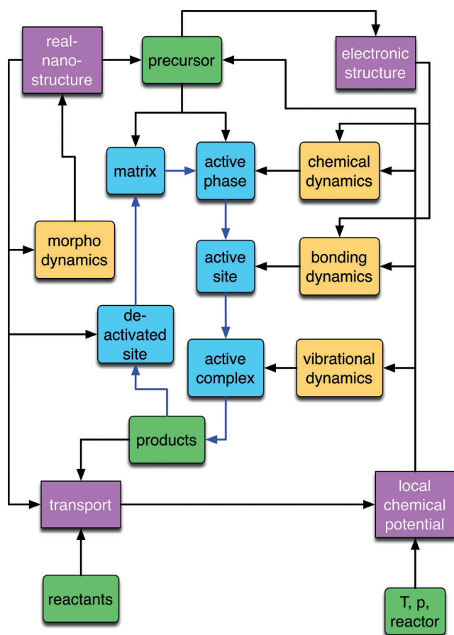
Figure 16. A realistic description of the feedback loop between the material chemistry of a heterogeneous catalyst and its function. The coloring elucidates different levels of chemistry and is clarified in the text.
