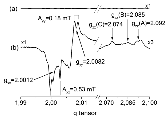
Figure 4. EPR spectra (X band) of MgO after heating in a vacuum at 1073 K. The measurement was performed at 77 K. For spectrum (a), only oxygen (50 mbar) was introduced, whereas for spectrum (b), oxygen and methane were introduced. Three different axial anisotropic environments can be seen for the hyperoxide radical.
