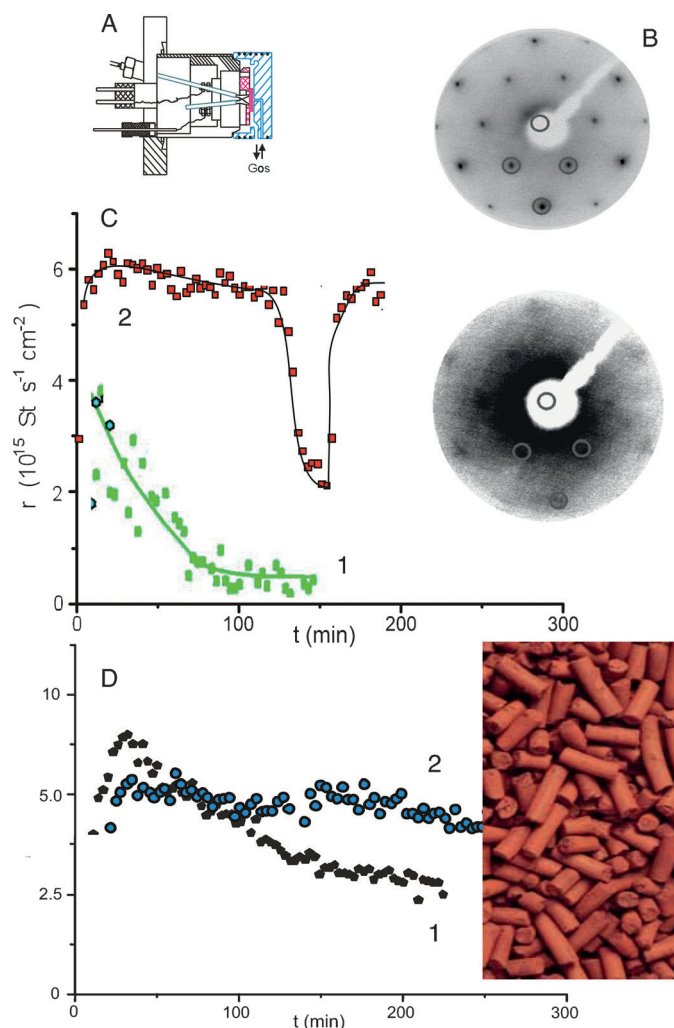
Figure 14. The dehydrogenation of EB to ST. A) Microreactor for the investigation of single crystals. B) LEED images (75 eV) from a \text{Fe}_2\text{O}_3 (111) surface before and after a reaction at 873 K with EB. C) Changes in the rate of EB consumption over time on a single-crystalline \text{Fe}_2\text{O}_3 catalyst; (1) only EB with water (1:10), (2) with EB and oxygen (1:10:0.5). D) As in (C) but with a polycrystalline \text{Fe}_2\text{O}_3 catalyst (optical image).
