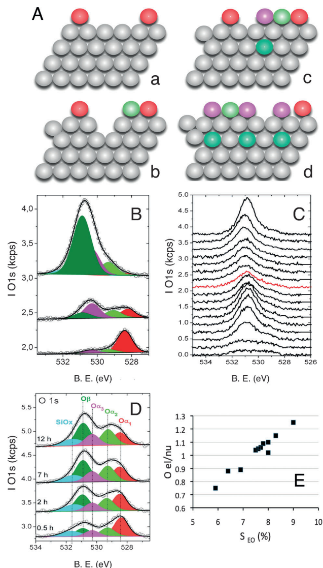
Figure 23. Several experimental results for silver as an oxidation catalyst. A) Stages of the interaction of oxygen with silver beginning at ca. 423 K. a) Adsorption and reconstruction, b) surface oxide and facilitated defect formation, c) as in (b) plus electrophilic oxygen through subsurface oxygen integration, d) surface oxide. The process of integration of oxygen into the bulk without the generation of an oxide proceeds much further at ca. 723 K, although only a small amount of adsorbed oxygen is available on the surface. B) XP spectra (O1s) of silver in 0.5 mbar oxygen: bottom: 2 h at 423 K, middle: 30 min at 723 K, top: 5 h at 723 K. C) XPS (O1s) desorption series of oxygen from the state (c) in (B). D) XPS (O1s) from silver particles (100 nm) in oxygen and ethylene (1:2, 0.5 mbar) at 503 K for the given times. E) Correlation of the proportions of the quantities of electrophilic (magenta and dark green in (D)) to nucleophilic (red, light green in (D)) oxygen versus the in situ observed selectivity to ethylene oxide. From Refs. [21b,339].
