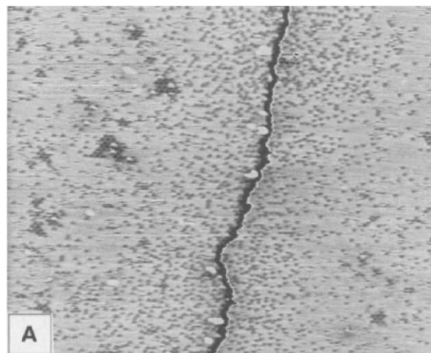
Figure 13. STM image of the decomposition of 0.3 L NO on (0001) Ru at 300 K after 30 min reaction time. The dark line depicts a top view of a monatomic step. From Ref. [130c].
