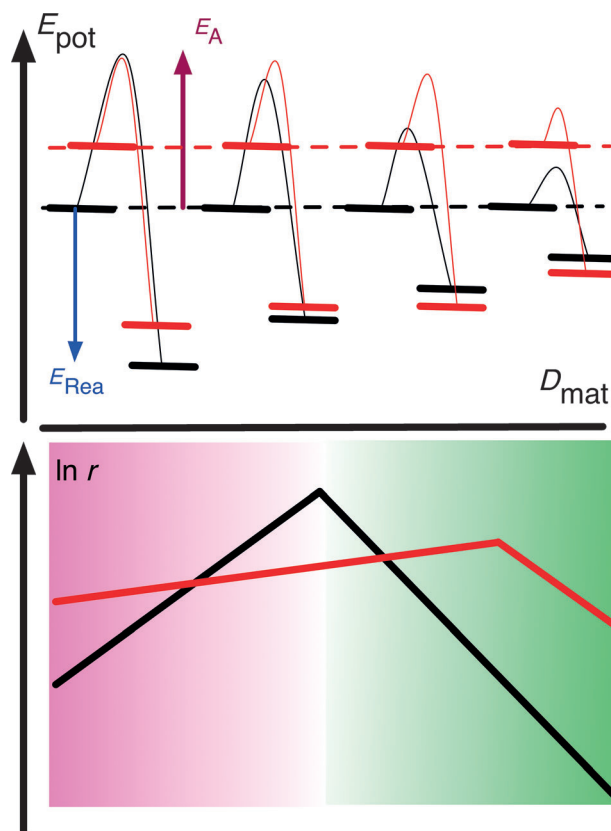
Figure 22. Relationship between the barrier height for the activation of a reactant and the strength of its interaction with a series of active phases (above) and the reaction rate of the corresponding catalytic conversion (below). The relation is shown for two reactants (red, black). The red field denotes the regions of the material descriptor ( D_{\text{mat}} ) in which the reactant is bonded too strongly to the catalyst, the green region shows where the interaction is too weak. E_{\text{Rea}} is the enthalpy of reaction of the rate-determining process, E_A is its activation barrier.
