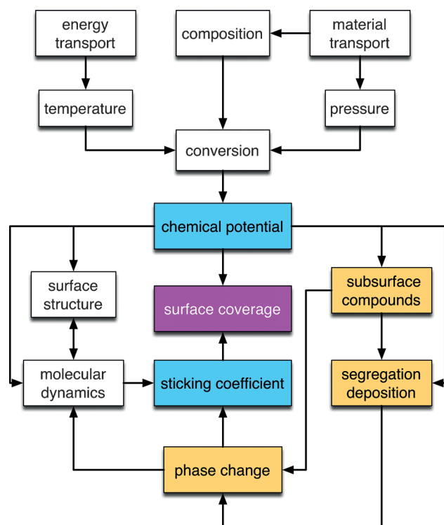
Figure 15. Influential factors that control the degree of surface coverage of a material in a heterogeneous reaction in the limiting case of high-performance conversion.
