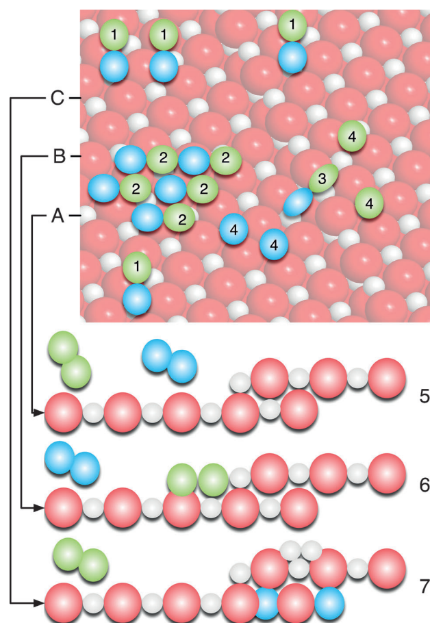
Figure 12. Simplified representation of the steps of a heterogeneous reaction according to the standard model. Steps (1)–(4) are shown in a top view of an ordered surface with two types of atoms and a monatomic step. They represent: (1) molecular adsorption, (2) island formation, (3) diffusion to the active center, and (4) dissociation. Steps (5)–(7) are shown as cross-section through the surface. The reactant is a diatomic molecule (blue/green). They represent: Reaction (A) desorption, reaction (B) desorption of a product and generation of a surface bond of the other product, (C) desorption of a product and the generation of a subsurface bond with the other product.
