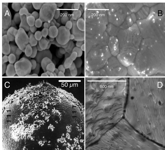
Figure 11. Catalytic etching in mesoscopic dimensions (in SEM). A–C) Silver in oxidation catalysis. The particles from (A) are completely sintered with one another after 100 h operation during the epoxidation of ethene at 523 K. Picture (B) shows the generation of crystal facets by the transport of bulk atoms: the small bright objects are particles of silicon contamination originally dissolved in the bulk that segregate as oxide. C) A single-crystalline sphere illustrating that catalytic etching is structure-sensitive and does not attack the (111) surface. The bright objects are relocated silver metal. D) Platinum, also after methanol oxidation. See Ref. [126]. Noticeable are the differing orientations of the grains that can be identified through the direction of the visible (111) facets.
