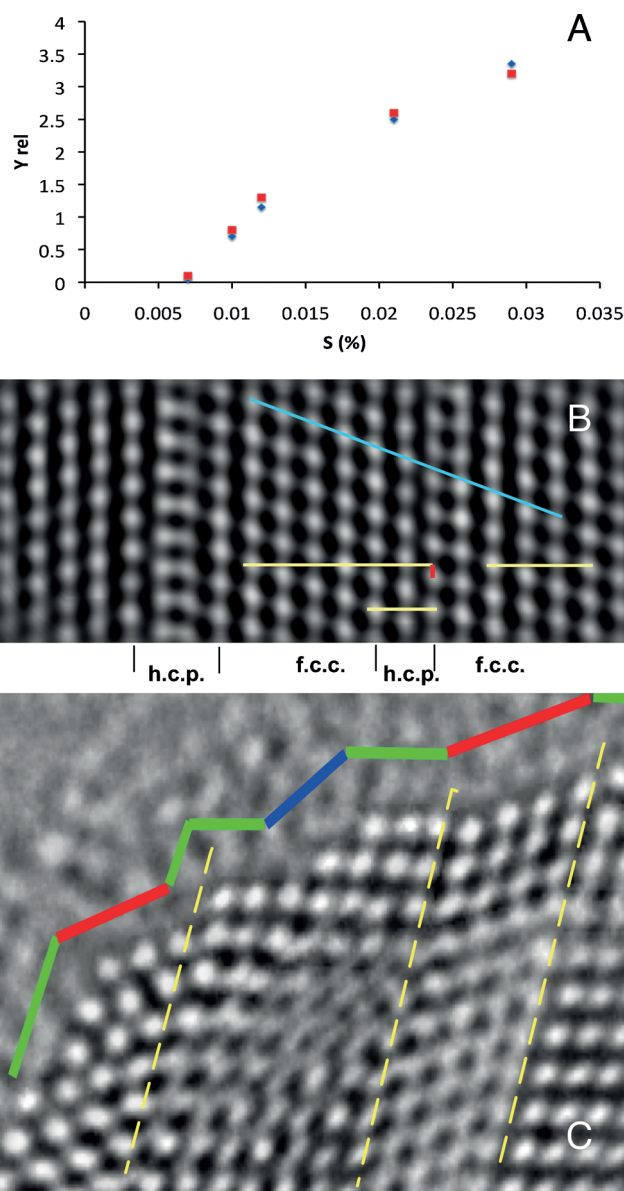
Figure 10. Structure–function relationship for Cu nanoparticles. A) Catalytic activity at 483 K (blue) and 523 K (red) in a stationary state for a stoichiometric reaction mixture at 60 bar pressure as [mass methanol/mass catalyst] × Cu surface area in arbitrary units. If the Cu surface were the controlling value, the result would be parallel to the x-axis. B) HR-TEM image of the interior of a Cu nanoparticle showing the dislocation in the stacking sequence of the atoms. The red line shows the dislocation of a row of atoms relative to the nominal position through the stacking sequence. C) Stacking errors effect a change in the surface termination of Cu nanoparticles. Three twin boundaries (yellow) change in distinct ways (red: (100), blue: (110), green: (111)). Taken from Ref. [56e].
