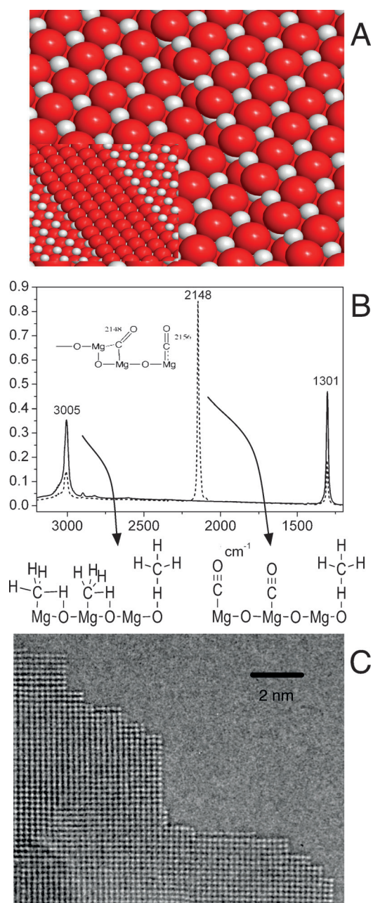
Figure 6. A) Model of a step in the (100) plane of MgO. The oxygen ions (red) are shown with a realistic size compared to the Mg 2+ ions (gray). A polar (111) step is displayed in the inset as a comparison. B) IR transmission spectrum of MgO after adsorption of methane (solid line) and after coadsorption of methane and CO (dashed line; measurement temperature 77 K, adsorption pressure 5 mBar). The schemes reflect the bonding arrangement of the adsorbates. C) Aberration-corrected TEM image of a MgO nanoparticle.
